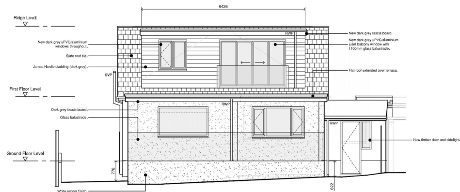
Proposed Rear Elevation 1:50
