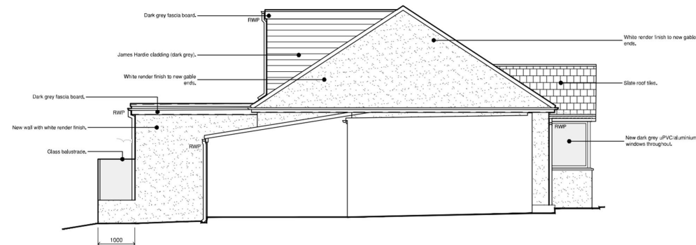
Proposed Side Elevation 1:50
