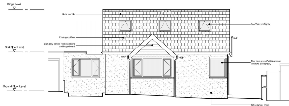
Proposed Front Elevation 1:50
