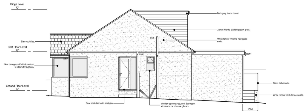
Proposed Side Elevation 1:50
